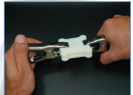
Figure 4. Clamping the mold before curing the silicone in oven.
