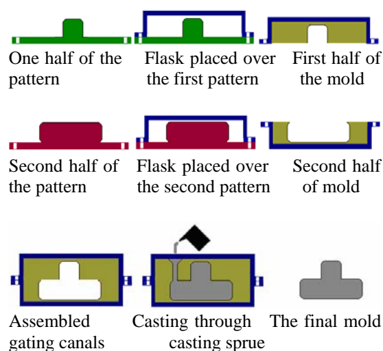
Figure 1: Workflow of the sand casting process
